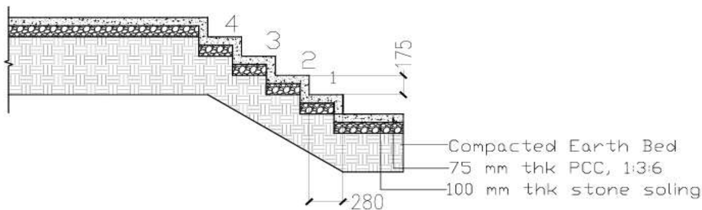
Elevation FOR RRM Staircase
