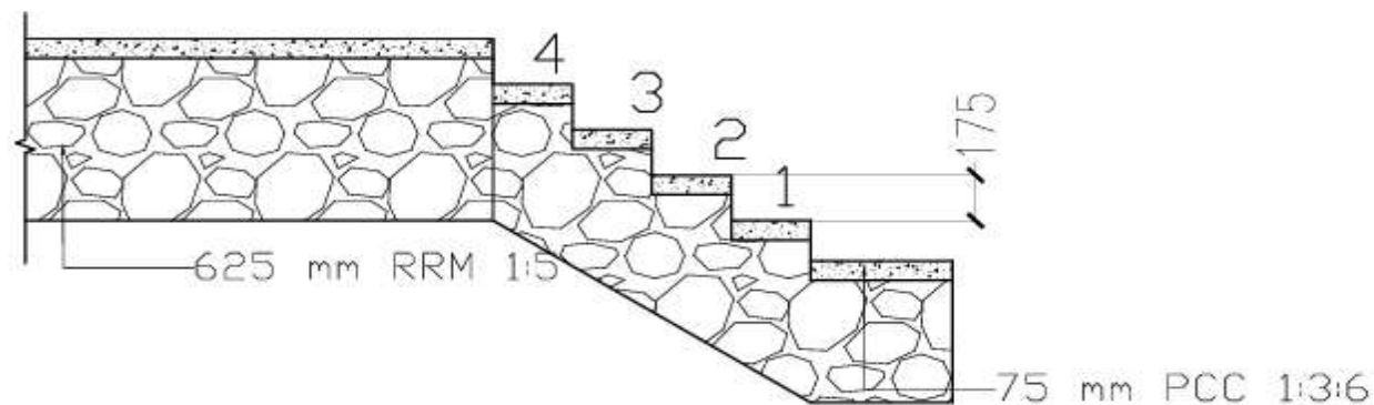
Elevation FOR RRM Staircase
